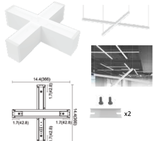
X Connector
