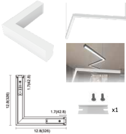
L Connector
