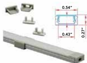
ZL-MC-1506 (-C OR -F) 4' aluminum mounting channel, Comes with 2 end caps and 2 mounting clips
