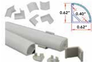
ZL-MC-1616 (-C OR -F) 4' aluminum mounting channel, Comes with 2 end caps and 8 mounting clips
