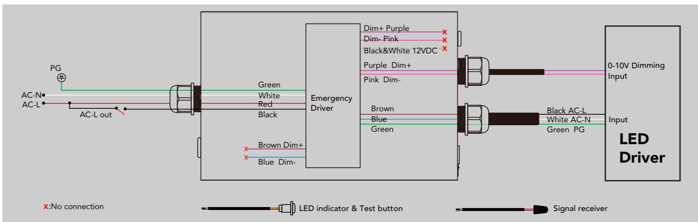
2. With Wall Switch ⚠ Driver Power ≥ Emergency Power
