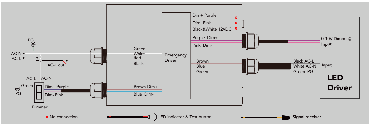
2. With Wall Switch ⚠ Driver Power ≥ Emergency Power
