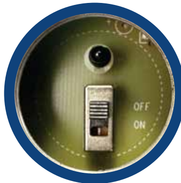
Photocontrol Selector
